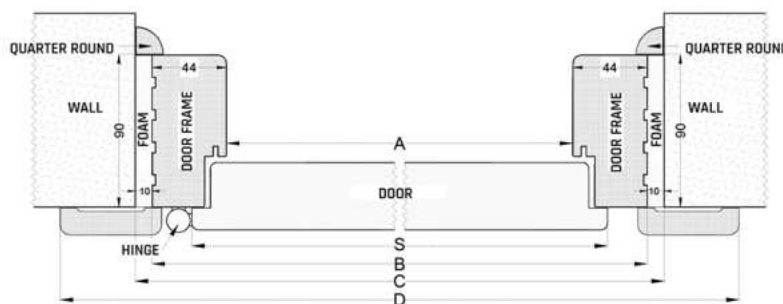
DIMENSIONS OF THE DOOR AND THE FIXED FRAME
